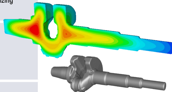
Temperature evolution during oil quenching
