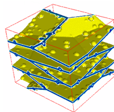
Grain boundary evolution and nucleation during forging
