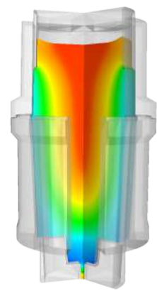
Temperature distribution during solidification
