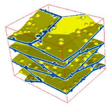
Grain boundary evolution and nucleation during forging
