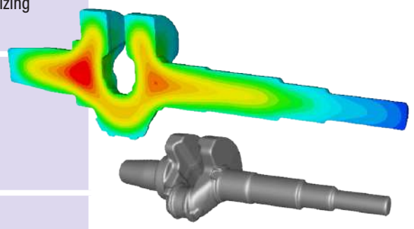
Temperature evolution during oil quenching
