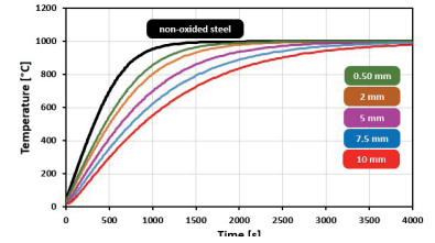
Influence of scale thickness on time required to homogenize the temperature at the center of the billet
